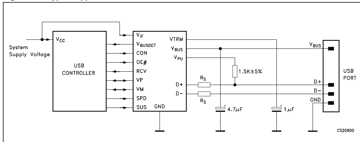
Figure 1. Typical application
